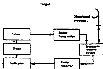
Fig. 1—PULSE RADAR SYSTEM.
